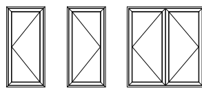
70mm Outerframe Low Wheel Chair Threshold Option
