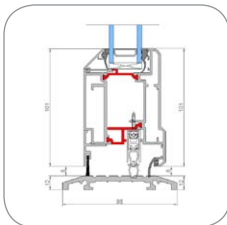
Cill Detail
